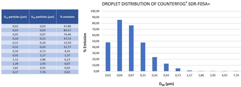
Fig. 6 Droplet distribution of COUNTERFOG® SDR-F05A+
